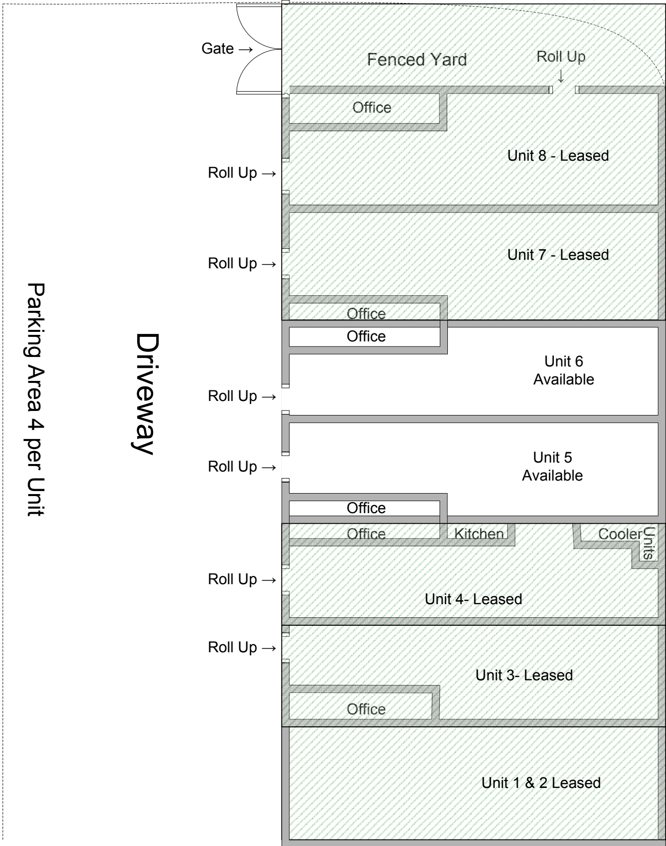
131 South Maple Building Plan
